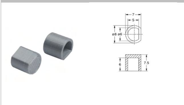
1352 Drehstangenadapter 8mm/6mm
