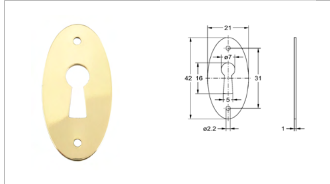
2106 Schlüsselschild
