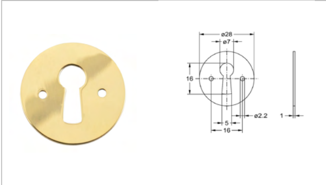
2107 Schlüsselschild
