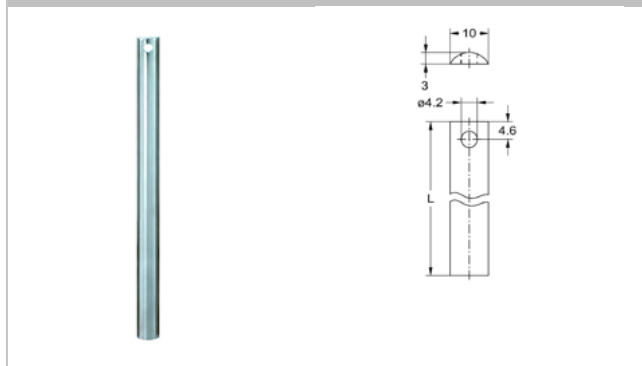
0103 Stange 10x3
