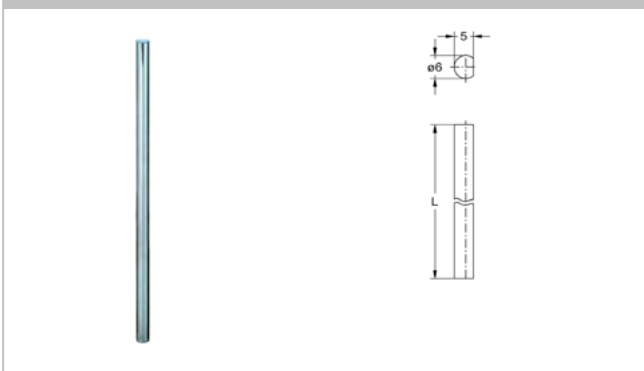
1352 Drehstangenadapter 8mm/6mm
